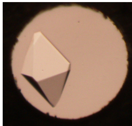
FIGURE 1 A single crystal of ice VI grown at 0.9 GPa and room temperature (diameter of the gasket hole is 0.3 mm). Ice XV, investigated by Komatsu et al. (2016), is a hydrogen-bond ordered form of ice VI.
