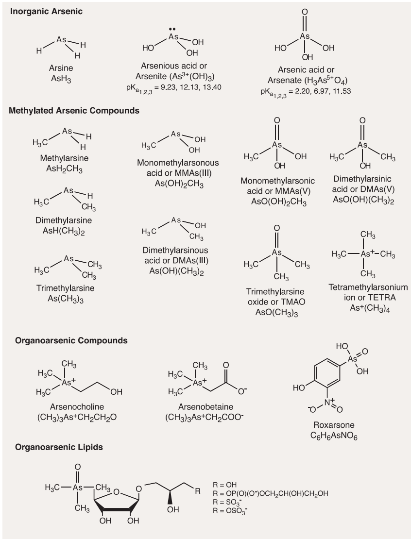
FIGURE 1 Summary of important inorganic, organic, and biological forms of arsenic in the environment. For inorganic aqueous species, stepwise acid dissociation constants ( \text{p}K_{a_n} = -\log(K_{a_n}) , where n is the number of protons dissociated and K_a is the equilibrium constant) are given. The position of lone-pair electrons are shown for inorganic \text{As}^{3+} . A wide variety of organoarsenic compounds and lipids have been identified; several of the major environmental species are shown here.
